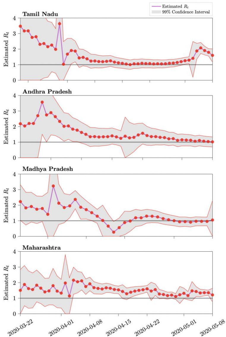
Figure 2. Estimated reproductive rate, by State
