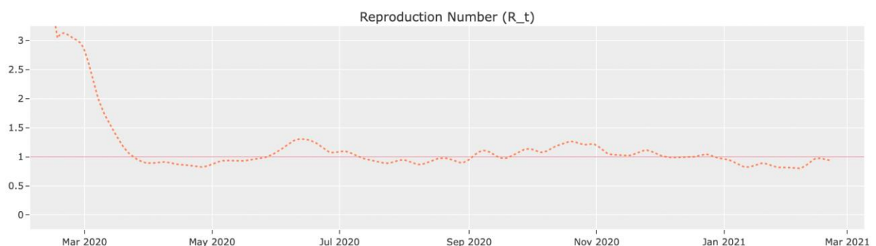
Figure 3. Effective reproduction number ( R_t ) for United States, March 2020-March 2021
